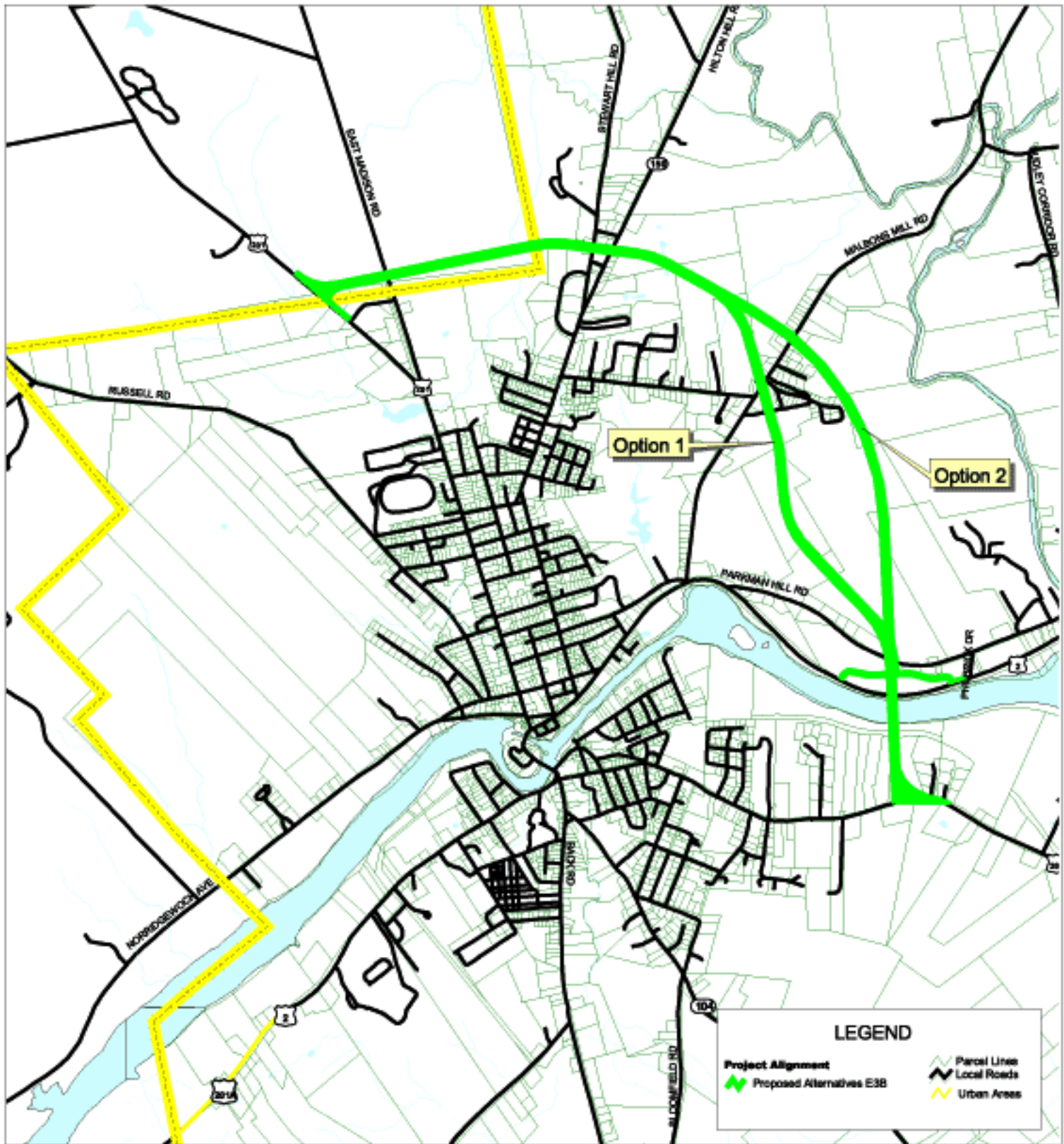
Skowhegan Transportation Plan Alternative E3B Figure 4
