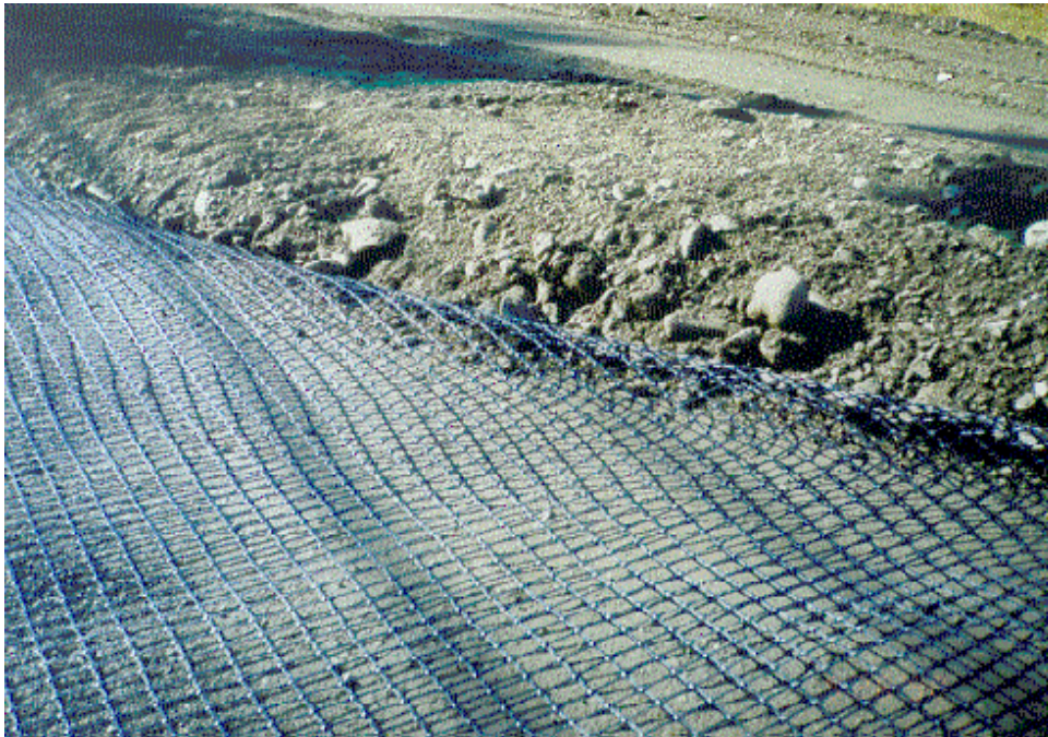
Photo 3: Geogrid Shoving
