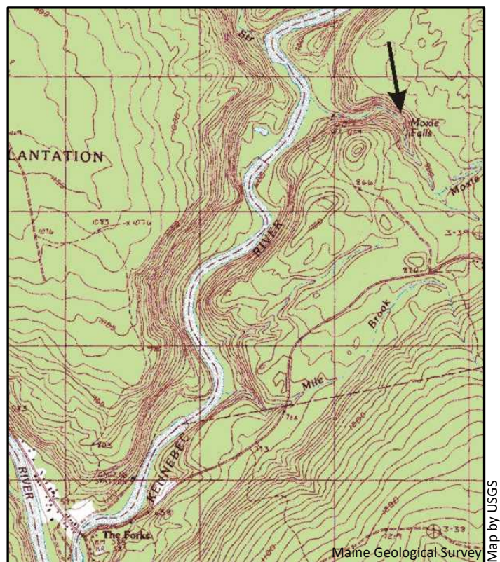
Figure 2. Topographic map showing location of Moxie Falls.
