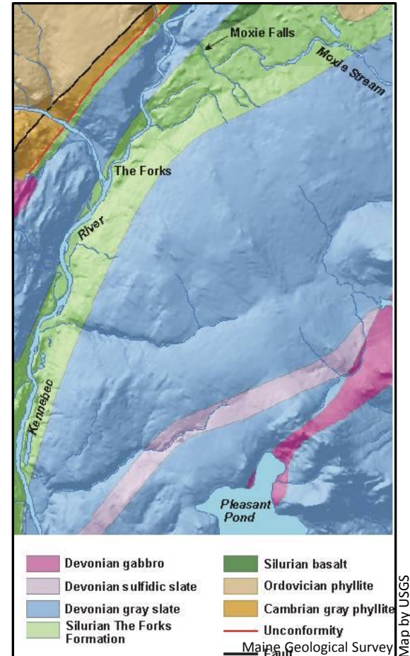
Figure 3. Generalized bedrock geologic map of The Forks quadrangle. The primary unit exposed at Moxie Falls is The Forks Formation of Silurian age in light green.
