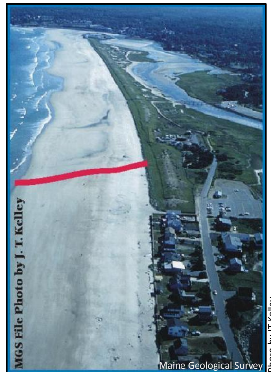
Figure 9. Approximate location of the beach profile line shown in Figure 10.
