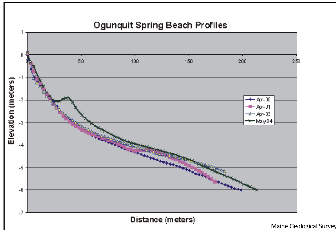
Figure 10. Comparison of spring beach profiles at the Ogunquit 2 station from April 2000 to May 2004.
