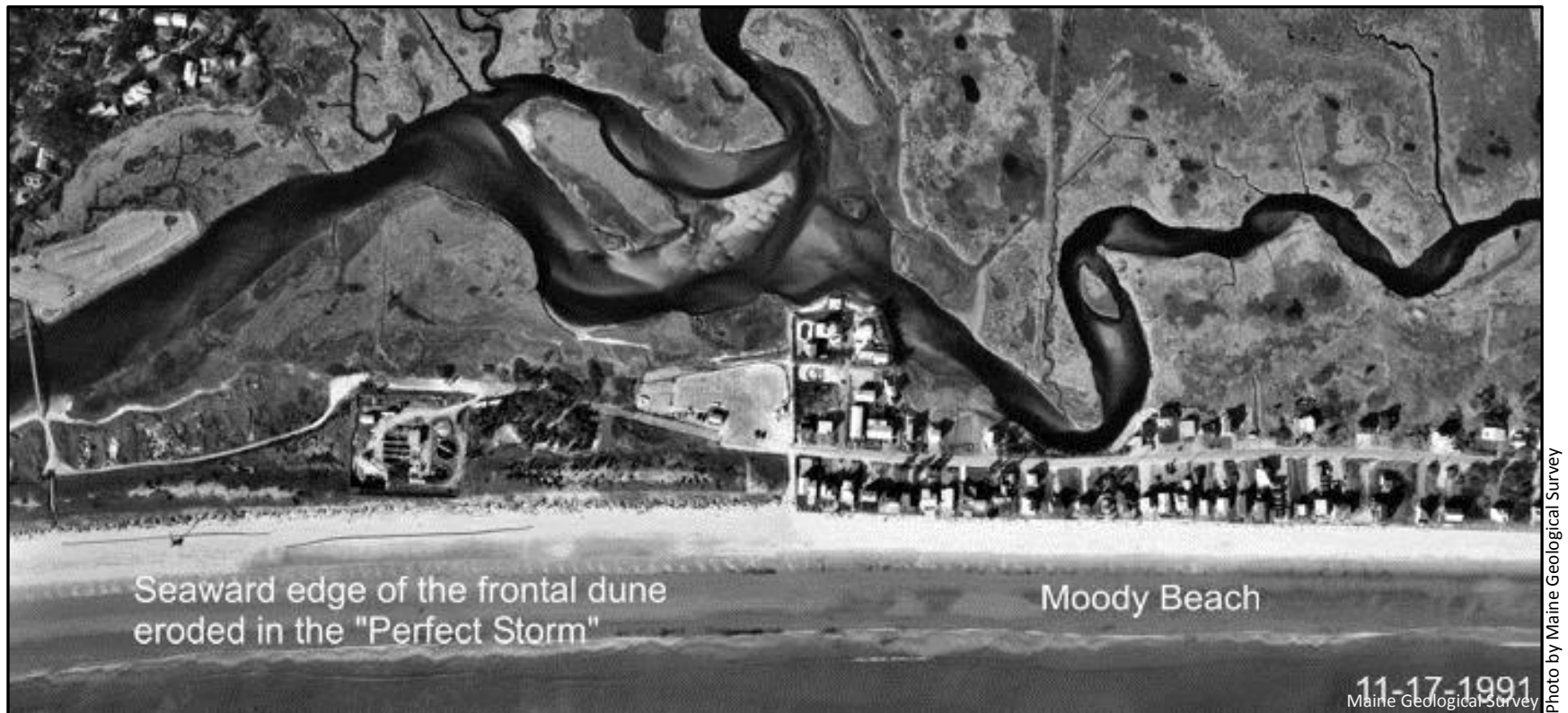
Figure 8. Aerial photograph of the seaward edge of the dunes in 1991 after the Perfect Storm.
