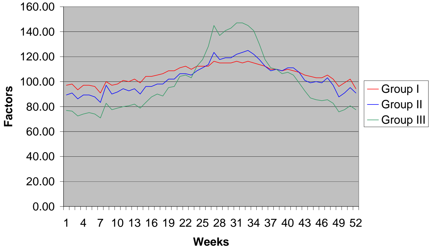
2009 Weekly Group Mean Factors as Percent of AADT Average: 2006, 2007, 2008
