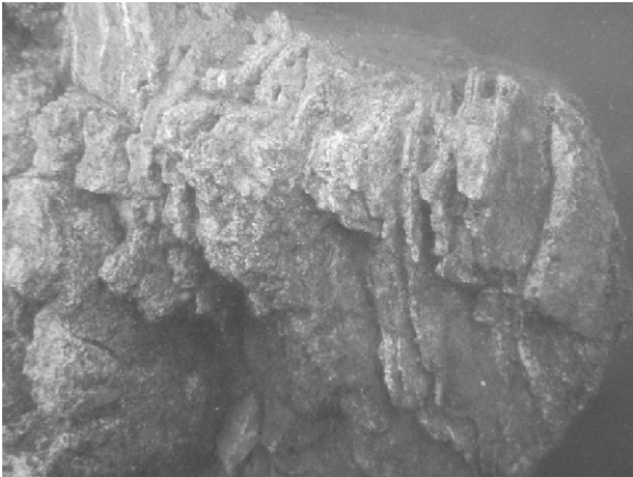
Parallel dikes with granitic intrusions.
