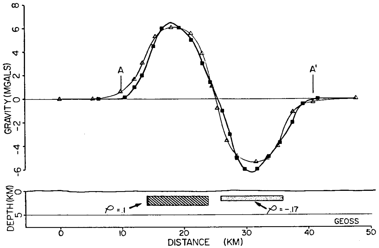
Figure 3.2-3. Gravity along the profile AA' in the Lisbon Falls area and preferred model of the subsurface distribution of rock. The density contrast for the granite, -0.17 \text{ gm/cm}^3 , is the value reported by Hodge et al. (1982) and also used by them for their model. The gravity values shown here are residual Bouguer gravity anomalies taken from Figure 3.1-6.
