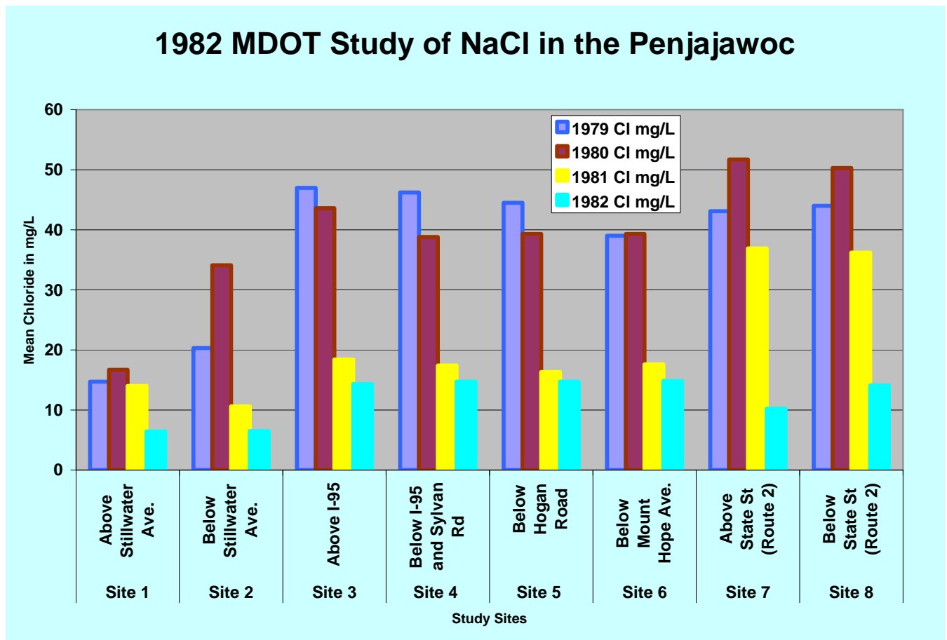
Figure 5. Summary of 1982 Maine DOT study of salt in Penjajawoc Stream. Values are yearly chloride means for each site. The sites are arranged from the upper watershed (left) to the lower watershed (right). The Bangor Mall is located between Sites 2 and 3. The DOT maintenance yard is between sites 6 and 7.
