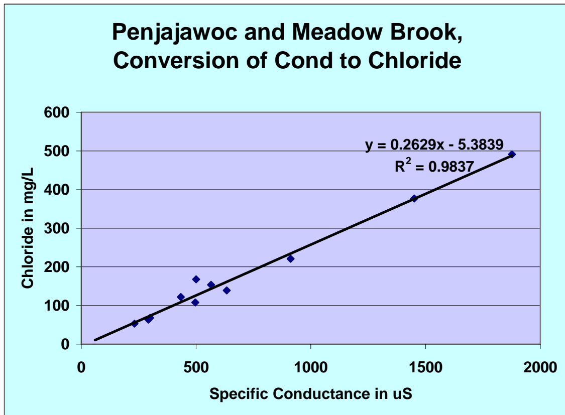
Figure 3. The results of a regression analysis of chloride in mg/l versus specific conductance in \mu\text{S} . The samples came from the lower Penjajawoc and from Meadow Brook. The R-square shows
