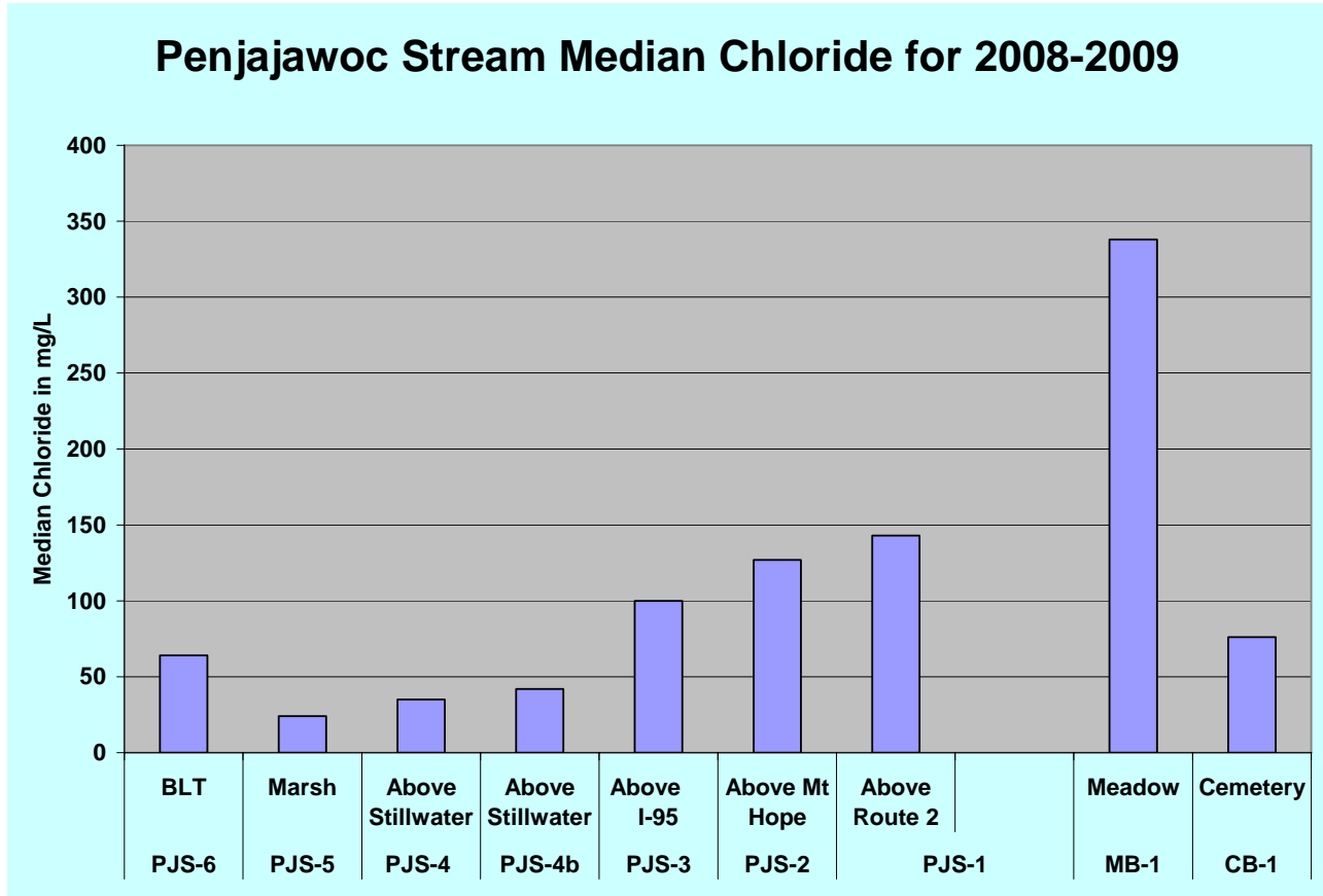
Figure 6. Graphic summary of Penjajawoc Stream estimated median chloride concentrations (based on the above regression). The sites are arranged from the upper watershed to the lowest, with the tributaries set off to the right.
