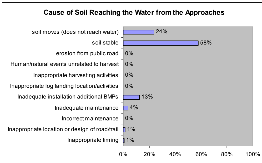
Figure 8 Causes of sedimentation from the approaches on sample units with crossings (n=277).
