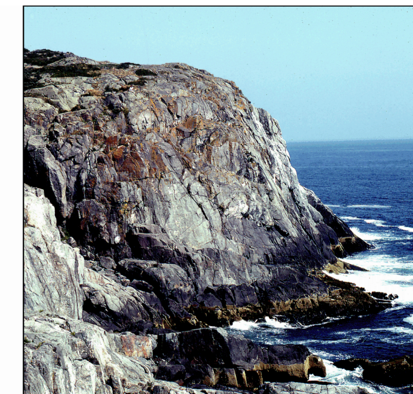
No bluff with a ledge shoreline. A steep slope on the bedrock surface is not a bluff. On this map, bluffs must be made of sedimentary material, generally with three feet or more relief. This shoreline type is very slow to change.
