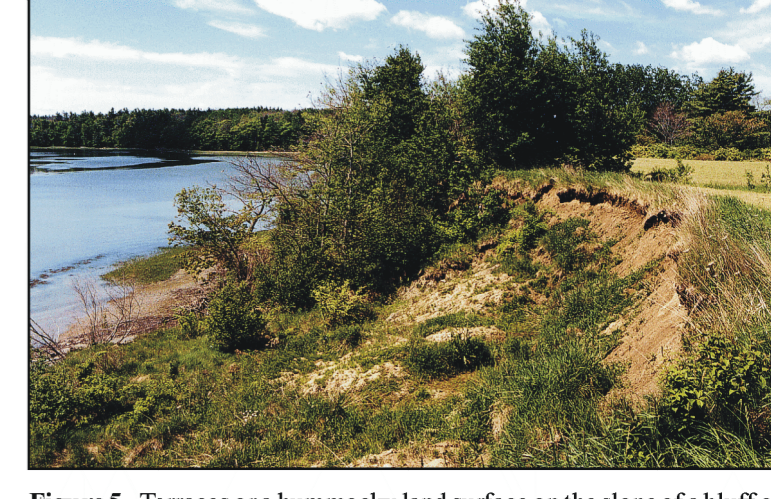
Figure 5. Terraces on a hummocky land surface on the slope of a bluff can indicate a former landslide. Terraces can be the surface of downslumped blocks which moved during a slide. Vegetation on the surface of these blocks may be tilted in various directions. The irregular land surface may also occur in a bowl-shaped depression below an arcuate top edge of the bluff, additional evidence of a former landslide.
