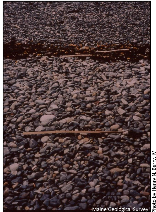
Figure 4. Stones in the lower part of the berm are smaller than stones in the upper part of the berm. Seaweed marks the upper limit of a storm deposit.
