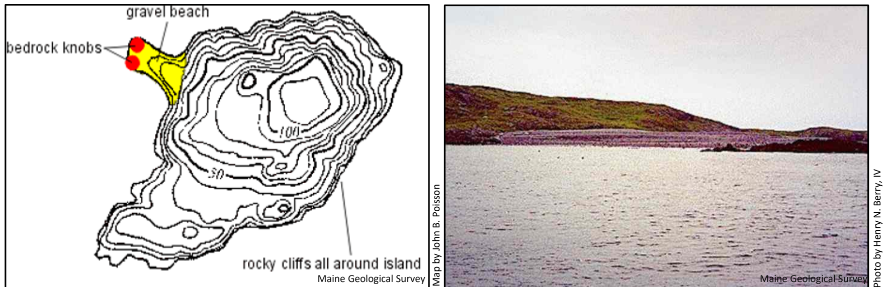
Figure 1. (Left) Map of a small island with a gravel beach. (Right) Pocket beach confined by main island to the left and small bedrock knob to the right.
