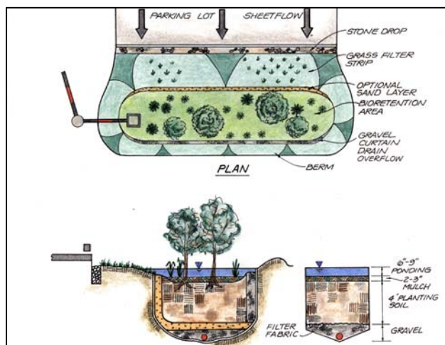
Figure 2: Schematic of a Bioretention System (Claytor & Schueler, 1996)
